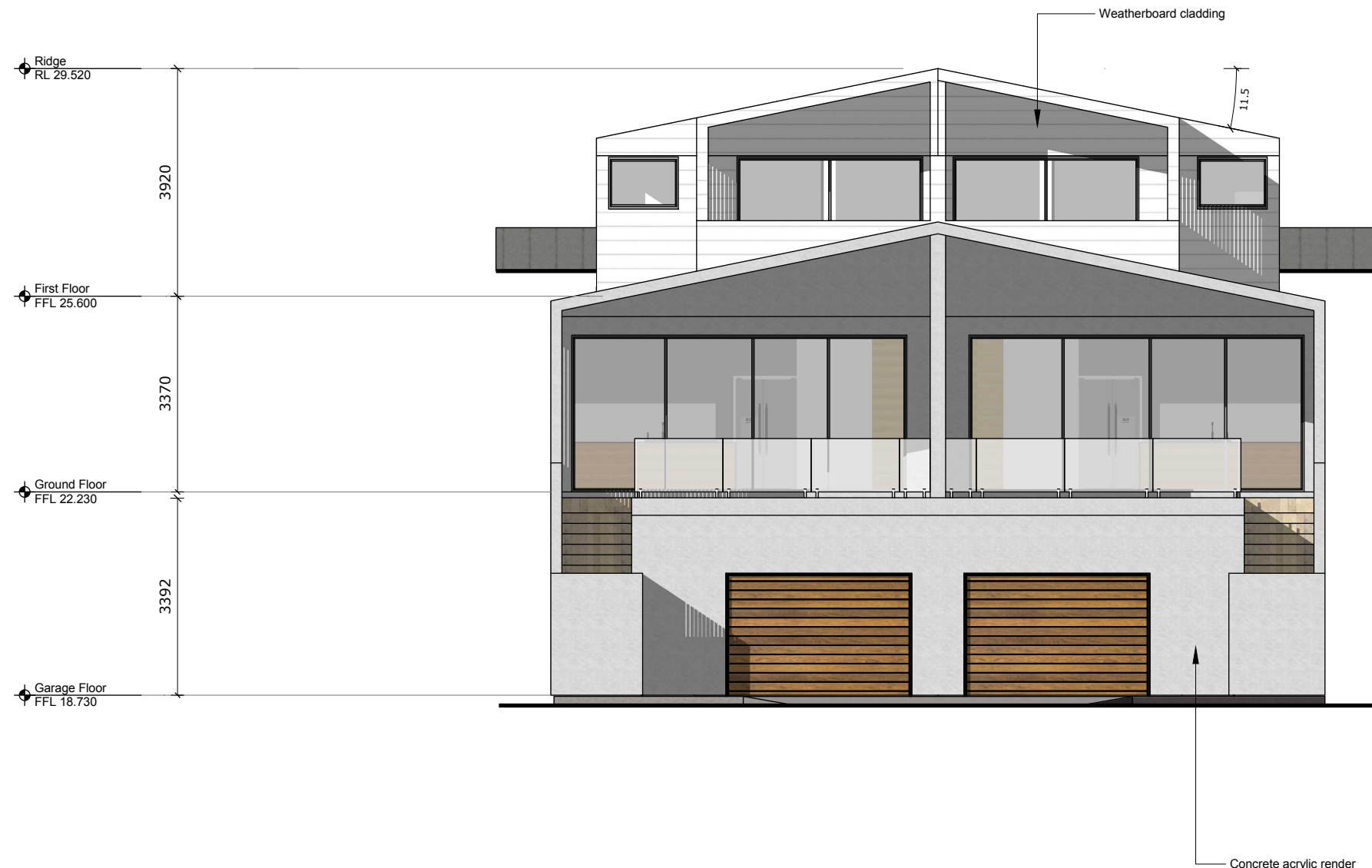
1 North Elevation Scale: 1 : 100
